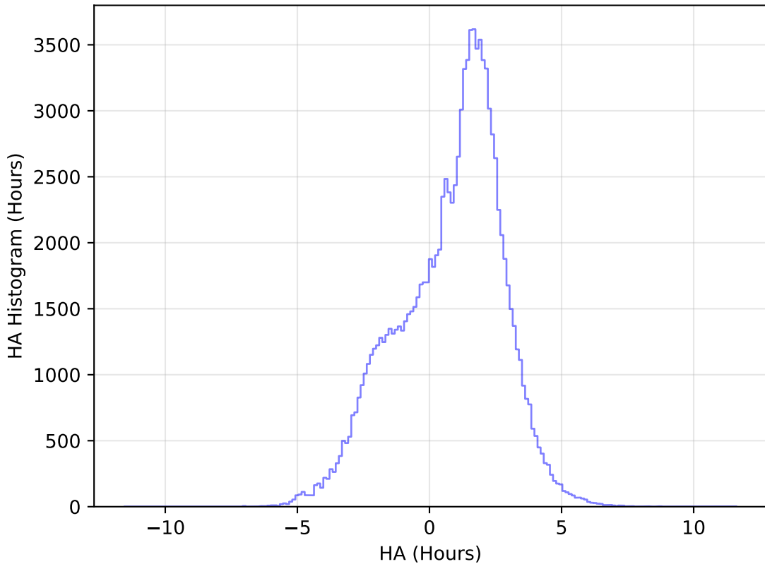
too_elab_heavy_r128_d3_griz_v3.4_10yrs All sky u band: HA Histogram
