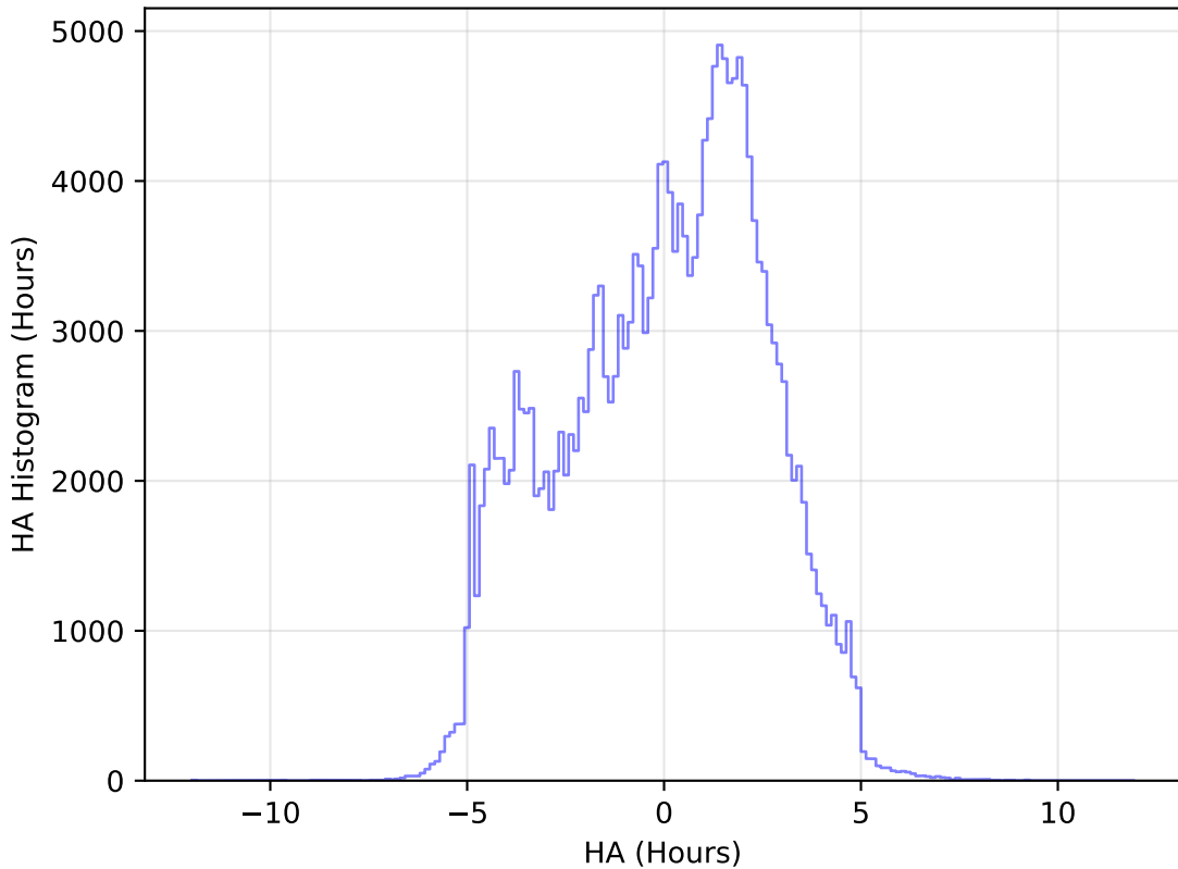
too_elab_heavy_r128_d3_griz_v3.4_10yrs All sky g band: HA Histogram
