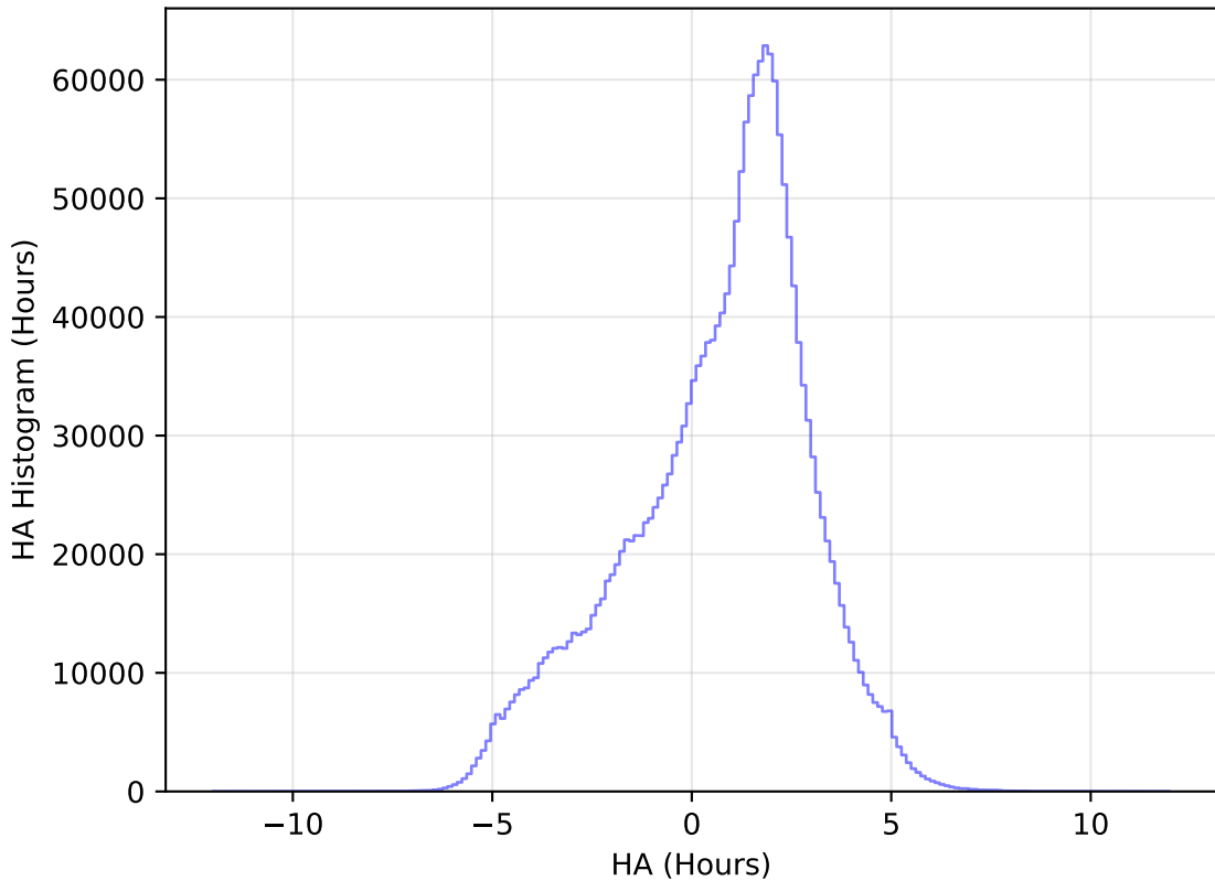
too_elab_heavy_r128_d3_griz_v3.4_10yrs All sky all bands: HA Histogram
