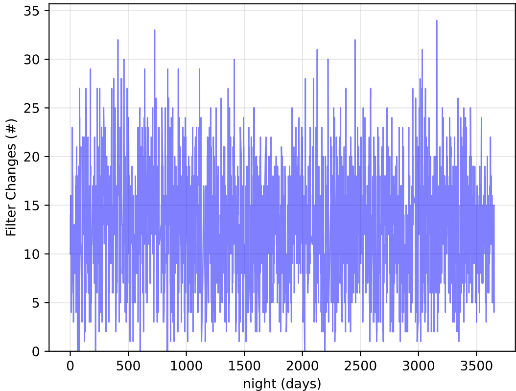
too_elab_heavy_r128_d3_griz_v3.4_10yrs Per Night: Filter Changes
