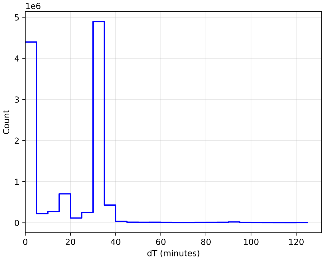
too_elab_heavy_r128_d3_griz_v3.4_10yrs WFD: DeltaT Histogram
