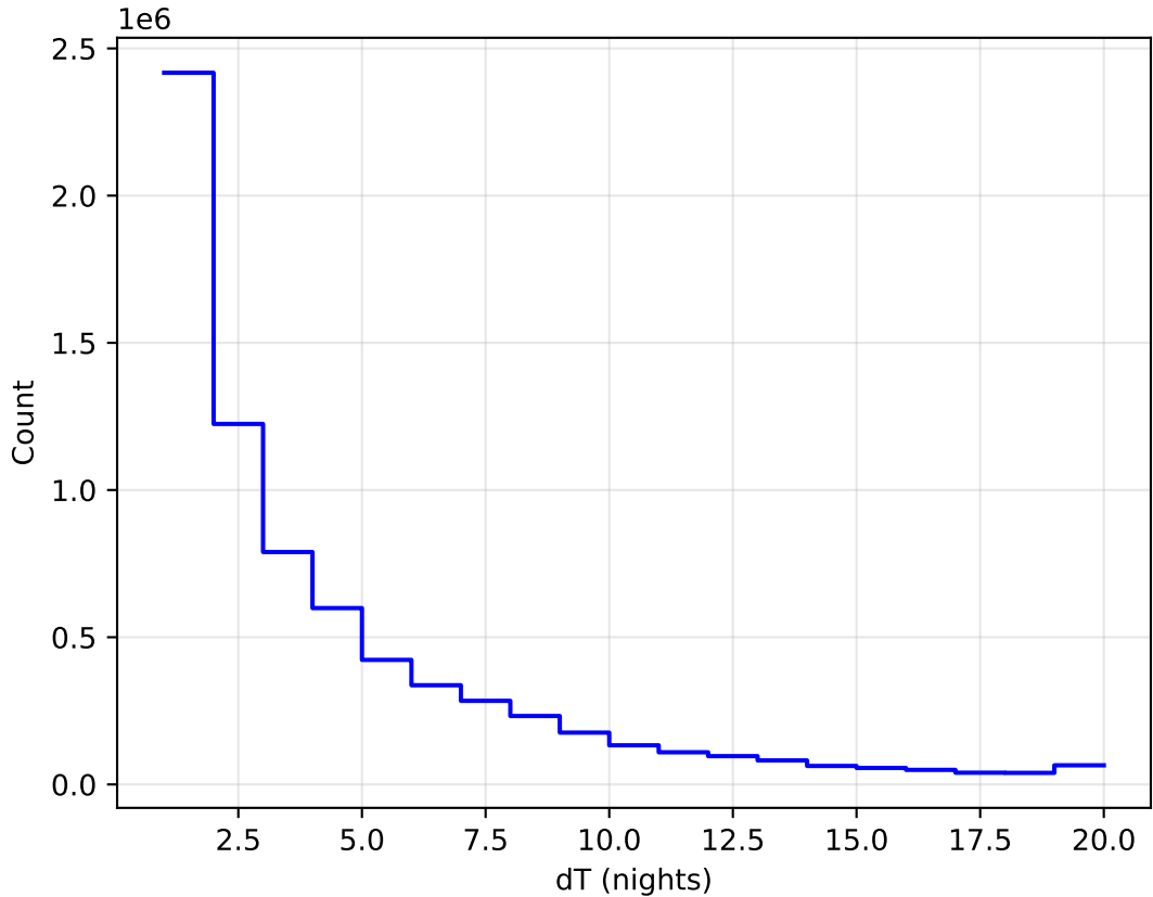
too_elab_heavy_r128_d3_griz_v3.4_10yrs WFD all bands: DeltaNight Histogram
