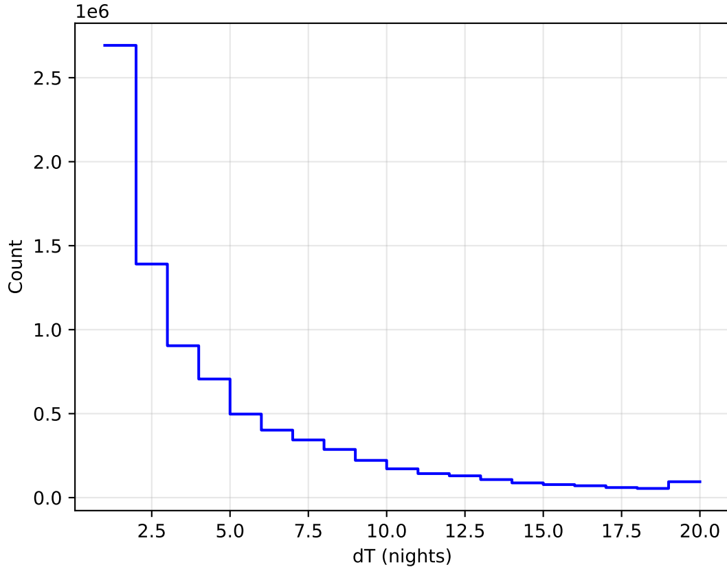
too_elab_heavy_r128_d3_griz_v3.4_10yrs All sky all bands: DeltaNight Histogram
