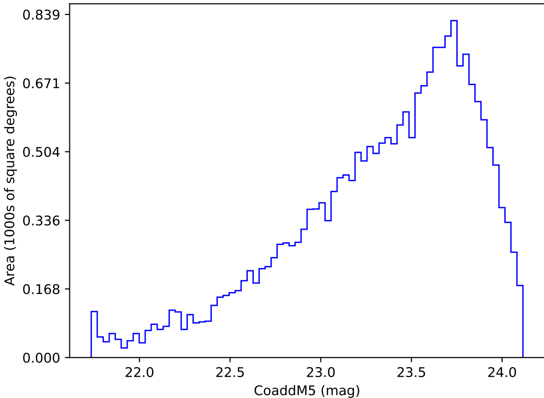
too_elab_heavy_r128_d3_griz_v3.4_10yrs Yr 3-4 y band: CoaddM5
