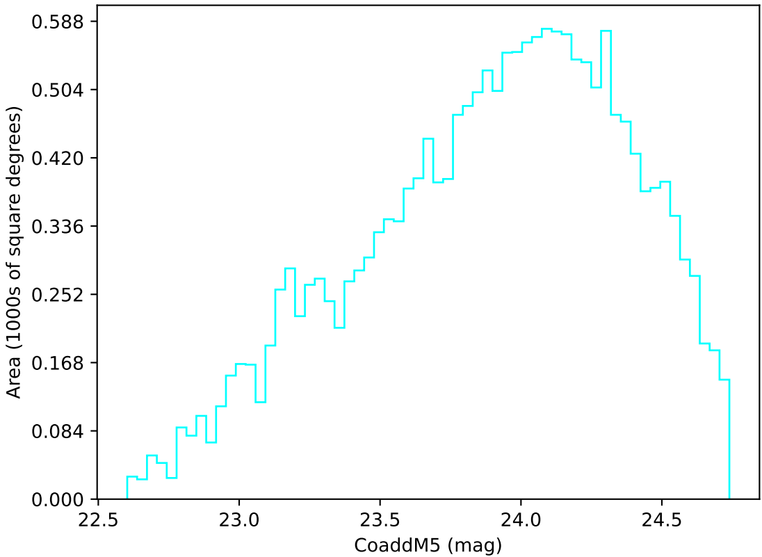
too_elab_heavy_r128_d3_griz_v3.4_10yrs Yr 3-4 u band: CoaddM5
