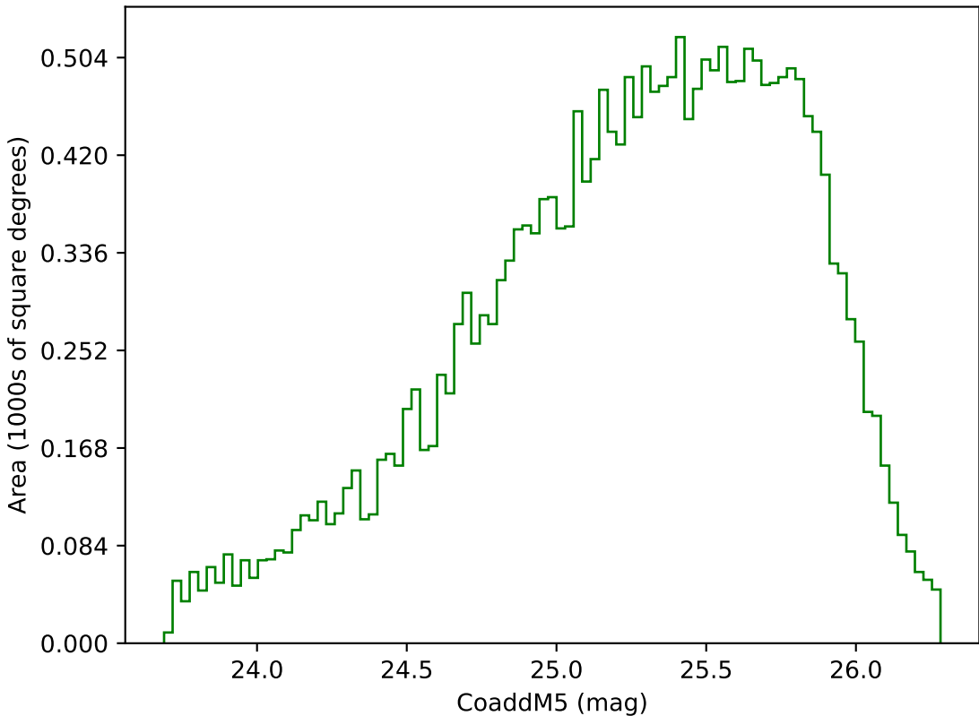
too_elab_heavy_r128_d3_griz_v3.4_10yrs Yr 3-4 g band: CoaddM5
