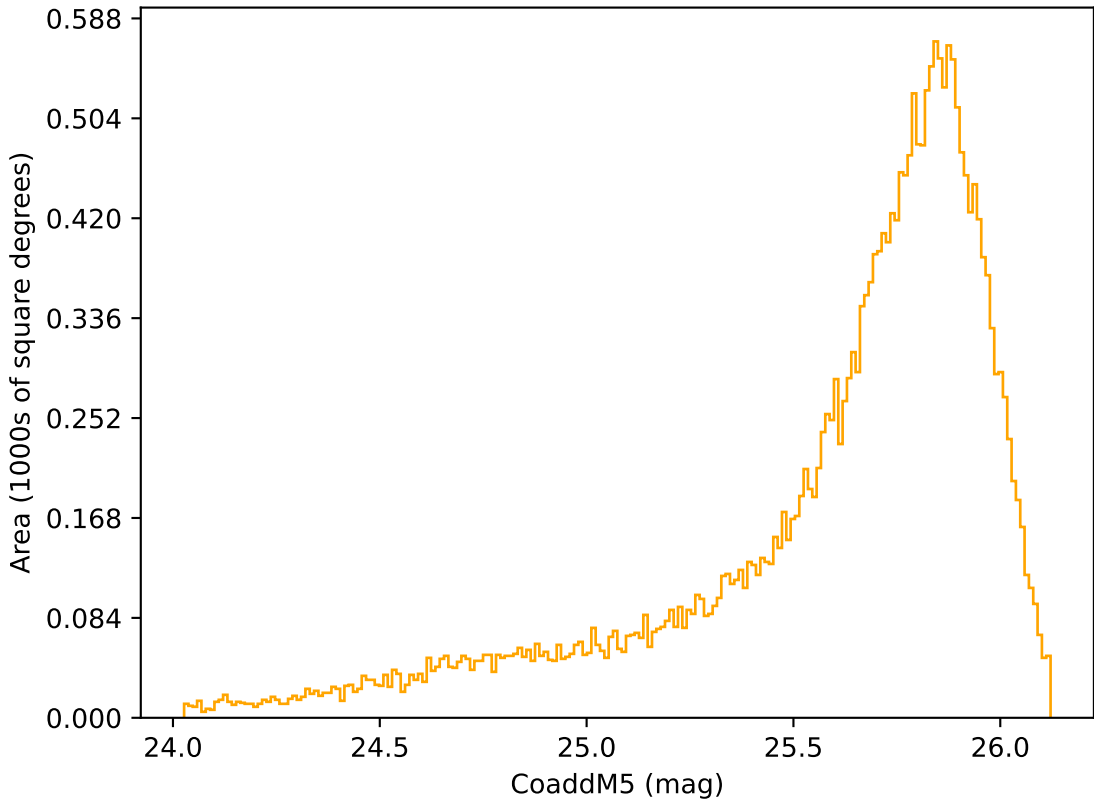
too_elab_heavy_r128_d3_griz_v3.4_10yrs Yr 1 r band: CoaddM5
