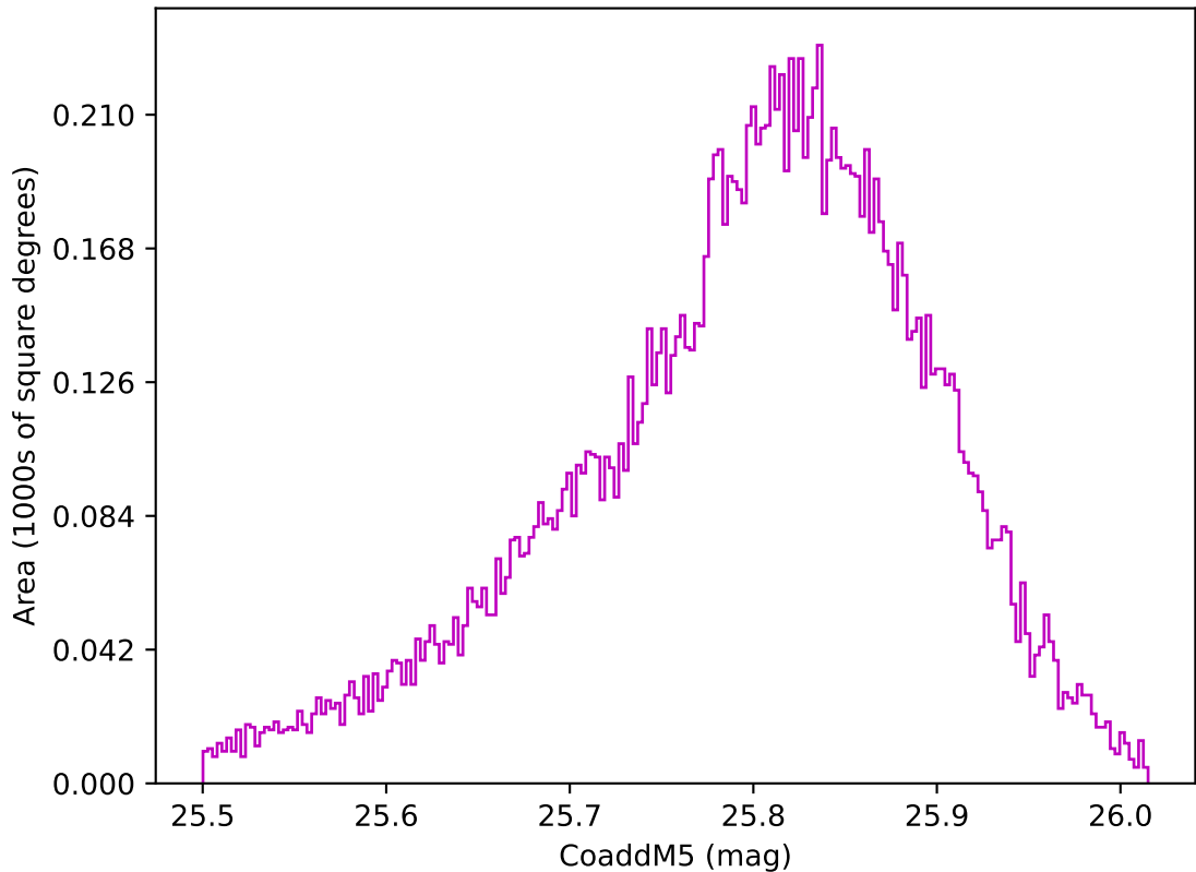
too_elab_heavy_r128_d3_griz_v3.4_10yrs WFD z band: CoaddM5
