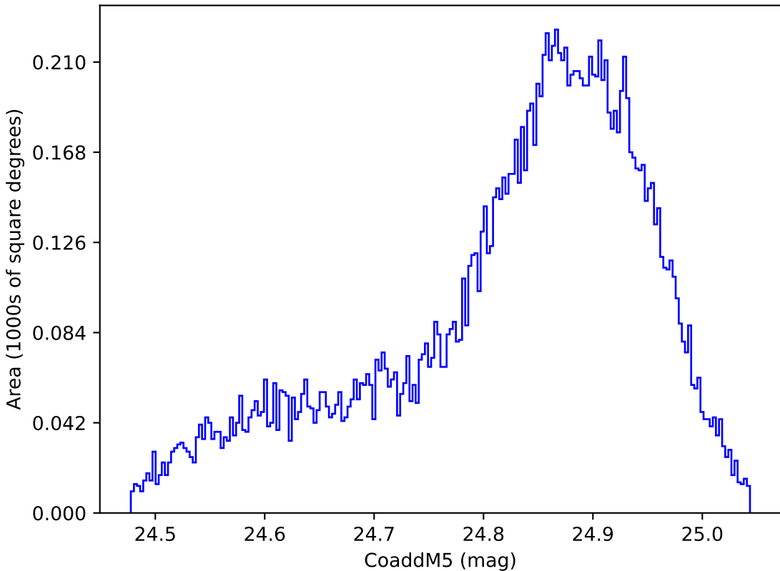
too_elab_heavy_r128_d3_griz_v3.4_10yrs WFD y band: CoaddM5
