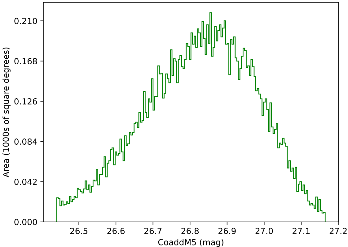
too_elab_heavy_r128_d3_griz_v3.4_10yrs WFD g band: CoaddM5
