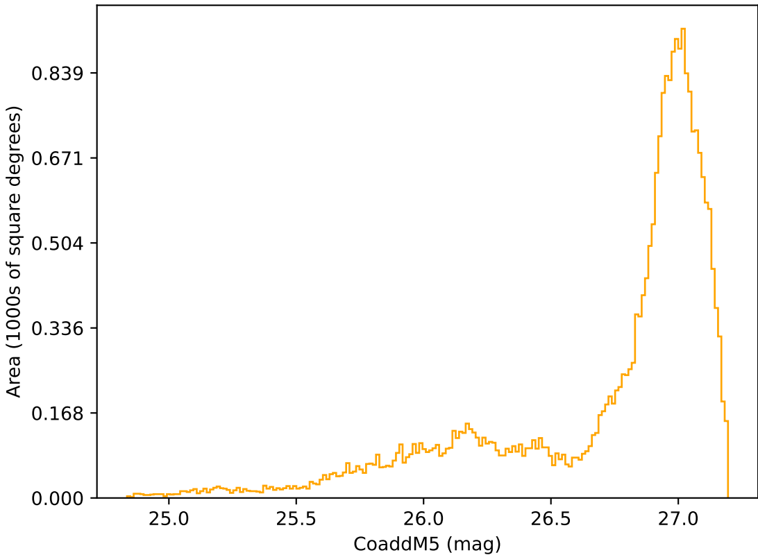
too_elab_heavy_r128_d3_griz_v3.4_10yrs All sky r band: CoaddM5
