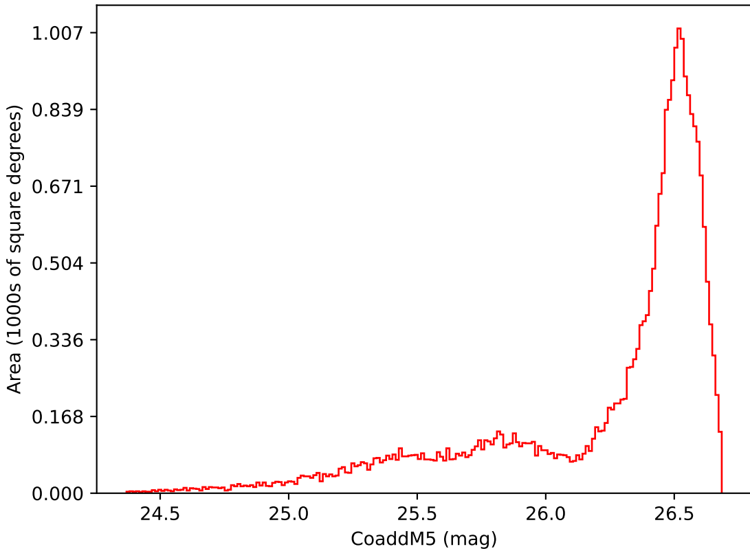
too_elab_heavy_r128_d3_griz_v3.4_10yrs All sky i band: CoaddM5
