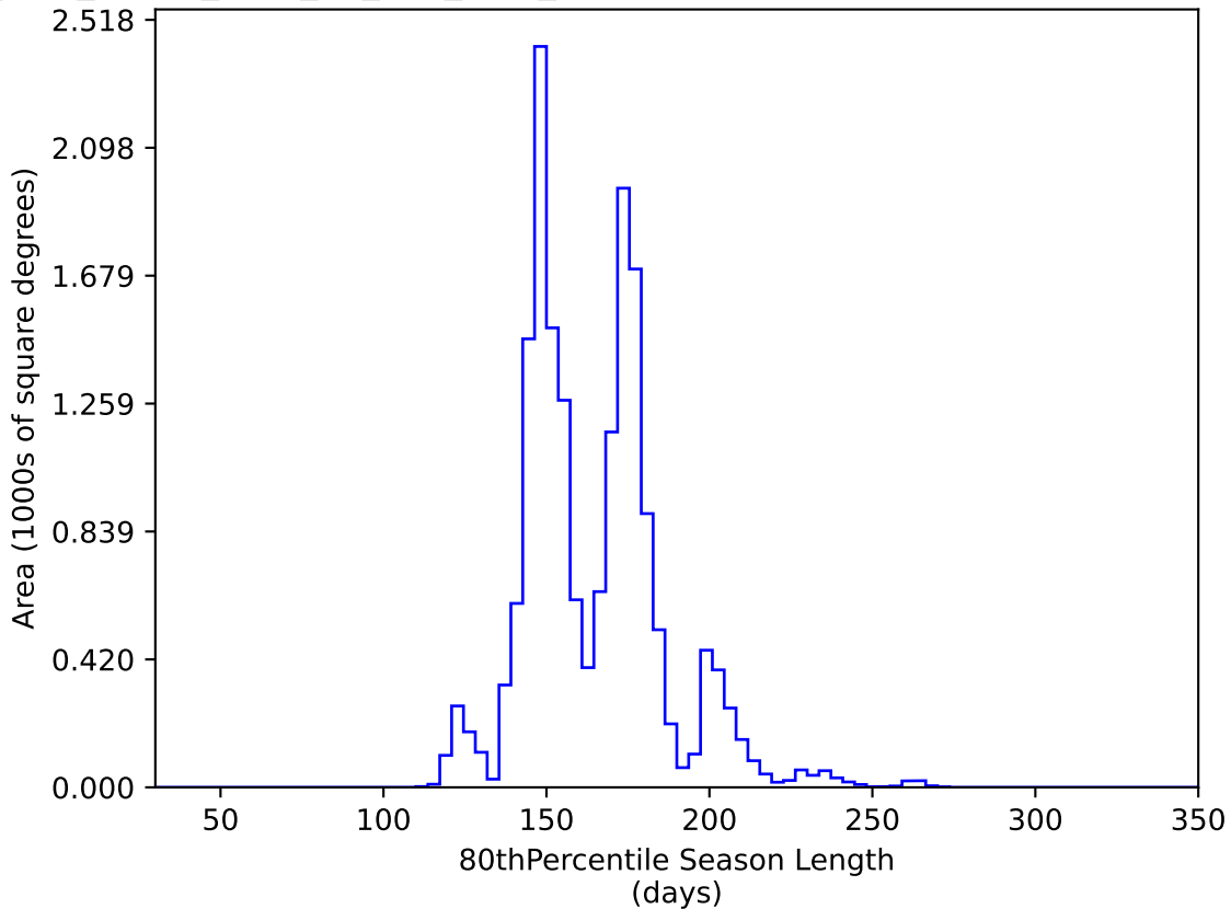
too_elab_heavy_r128_d3_griz_v3.4_10yrs WFD y band: 80thPercentile Season Length
