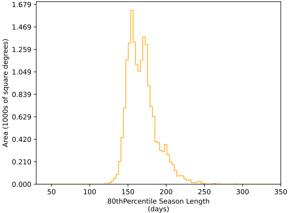
too_elab_heavy_r128_d3_griz_v3.4_10yrs WFD r band: 80thPercentile Season Length
