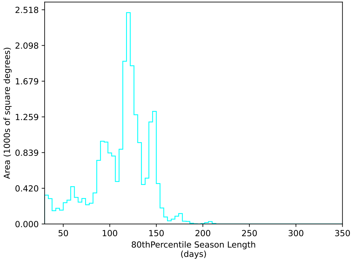
too_elab_heavy_r128_d3_griz_v3.4_10yrs All sky u band: 80thPercentile Season Length
