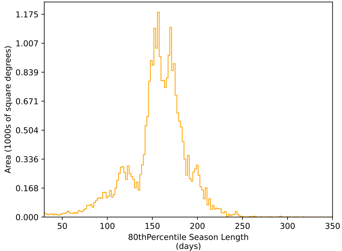
too_elab_heavy_r128_d3_griz_v3.4_10yrs All sky r band: 80thPercentile Season Length
