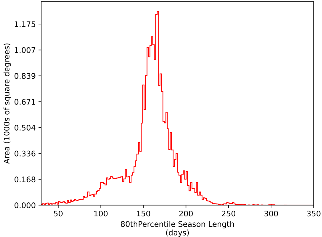
too_elab_heavy_r128_d3_griz_v3.4_10yrs All sky i band: 80thPercentile Season Length
