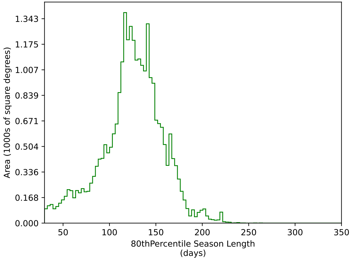
too_elab_heavy_r128_d3_griz_v3.4_10yrs All sky g band: 80thPercentile Season Length
