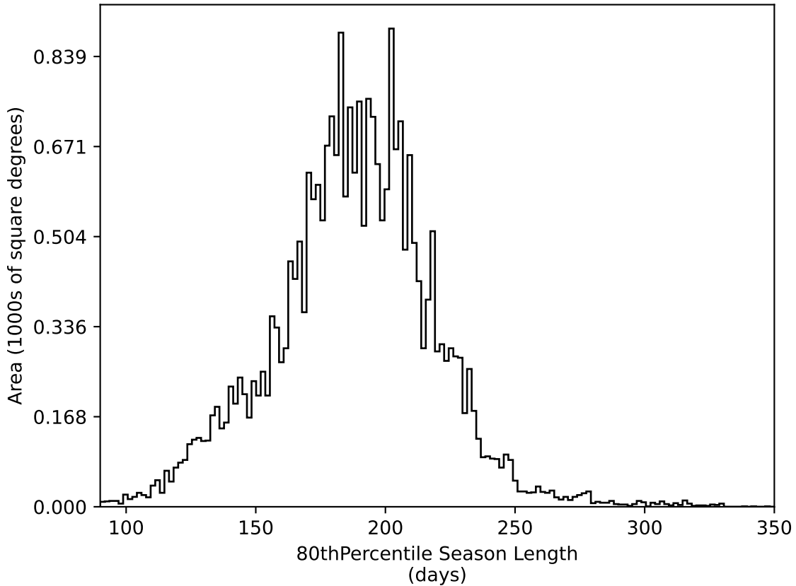
too_elab_heavy_r128_d3_griz_v3.4_10yrs All sky all bands: 80thPercentile Season Length
