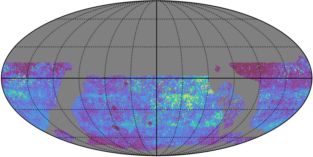
too_elab_heavy_r128_d3_griz_v3.4_10yrs WFD y band: 75th Percentile Intranight Timespan
