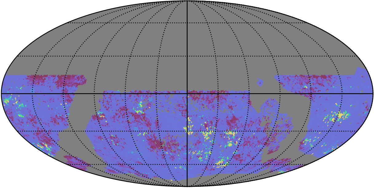
too_elab_heavy_r128_d3_griz_v3.4_10yrs WFD ug bands: 75th Percentile Intranight Timespan
