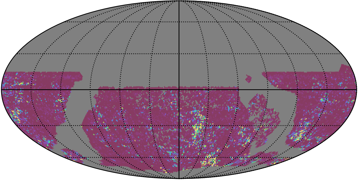
too_elab_heavy_r128_d3_griz_v3.4_10yrs WFD u band: 75th Percentile Intranight Timespan
