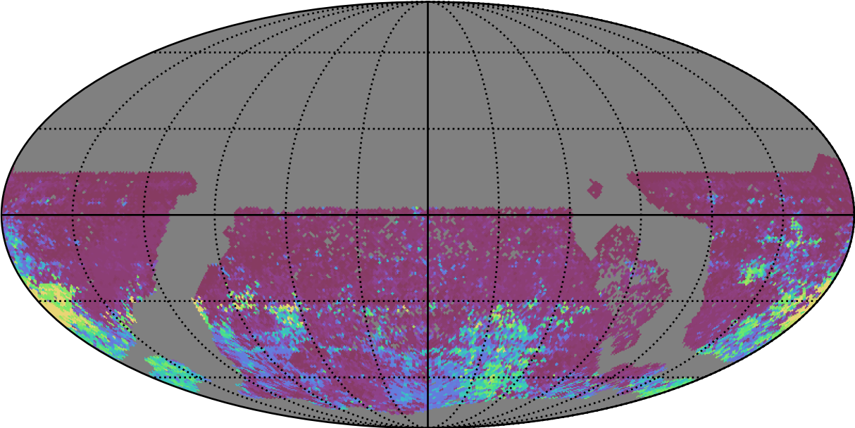
too_elab_heavy_r128_d3_griz_v3.4_10yrs WFD r band: 75th Percentile Intranight Timespan
