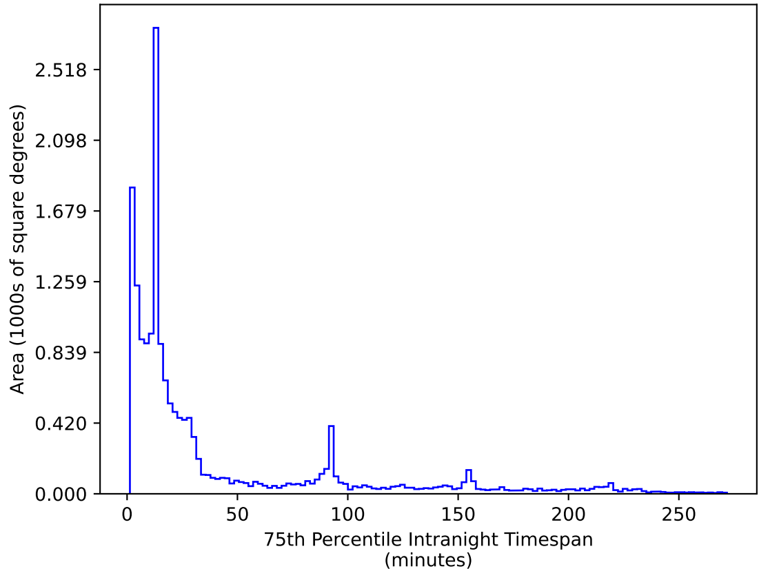
too_elab_heavy_r128_d3_griz_v3.4_10yrs WFD r band: 75th Percentile Intranight Timespan
