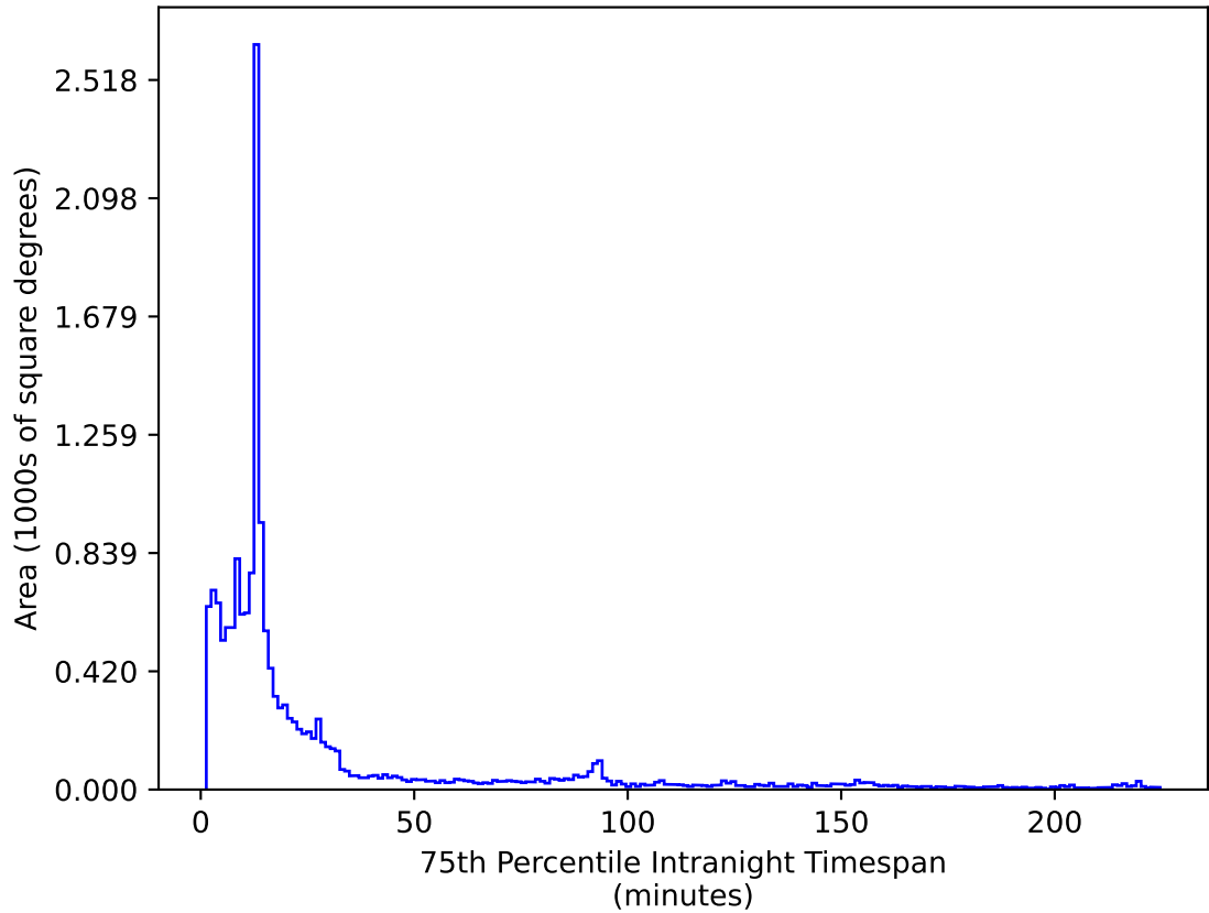
too_elab_heavy_r128_d3_griz_v3.4_10yrs WFD i band: 75th Percentile Intranight Timespan
