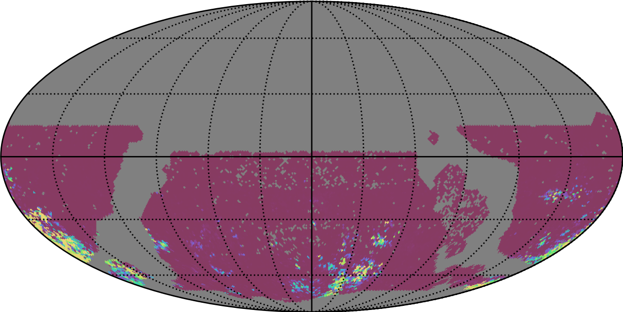
too_elab_heavy_r128_d3_griz_v3.4_10yrs WFD gr bands: 75th Percentile Intranight Timespan
