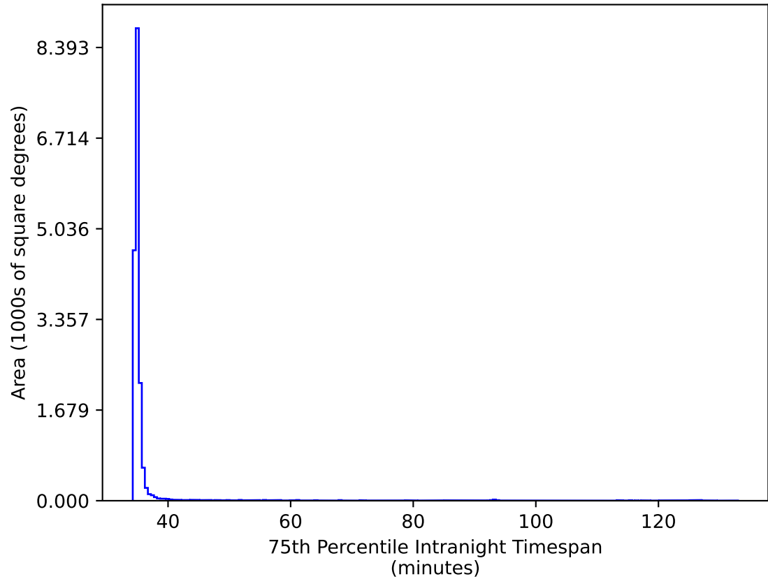
too_elab_heavy_r128_d3_griz_v3.4_10yrs WFD gr bands: 75th Percentile Intranight Timespan
