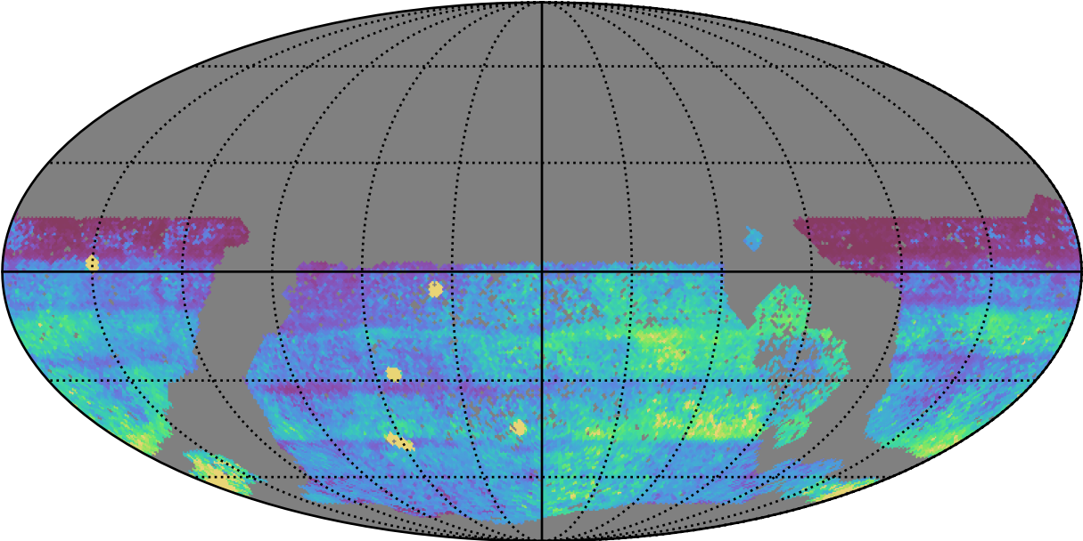
too_elab_heavy_r128_d3_griz_v3.4_10yrs WFD all bands: 75th Percentile Intranight Timespan
