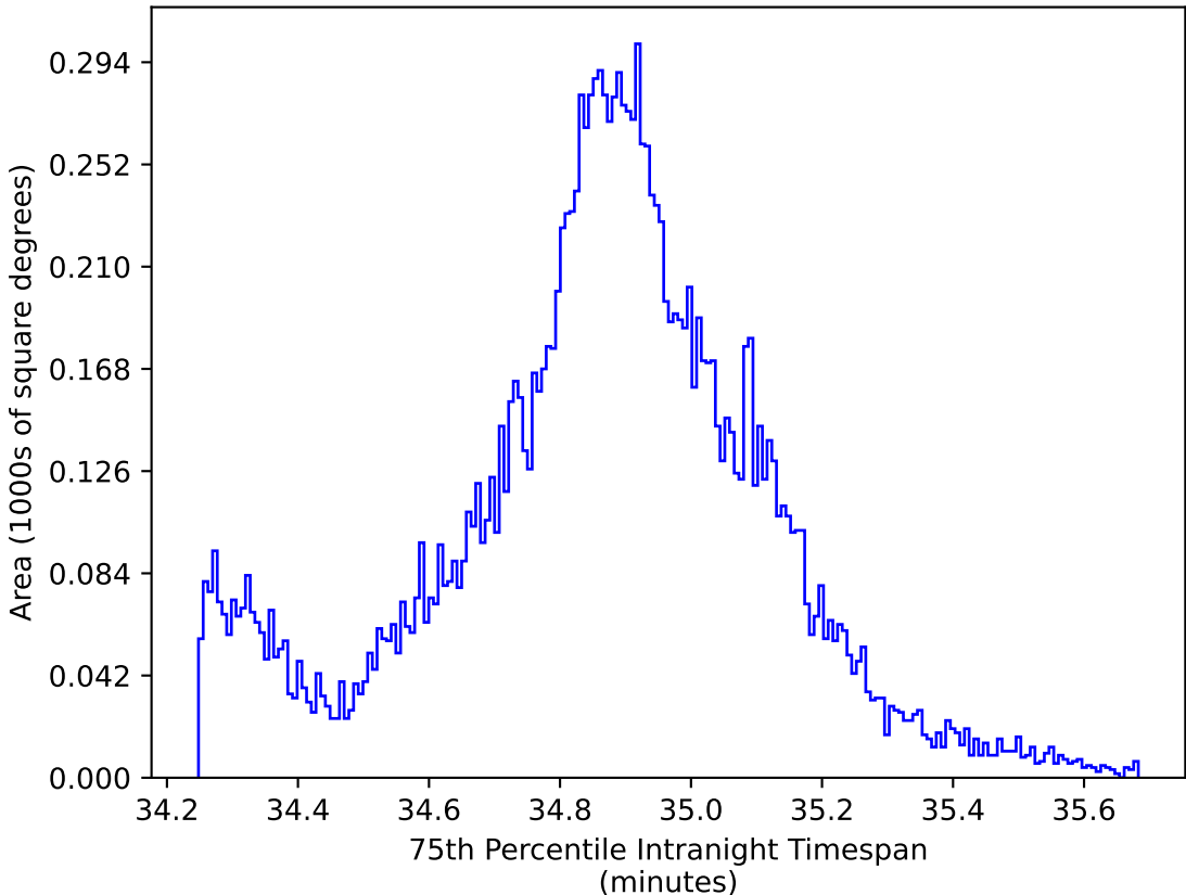
too_elab_heavy_r128_d3_griz_v3.4_10yrs WFD all bands: 75th Percentile Intranight Timespan
