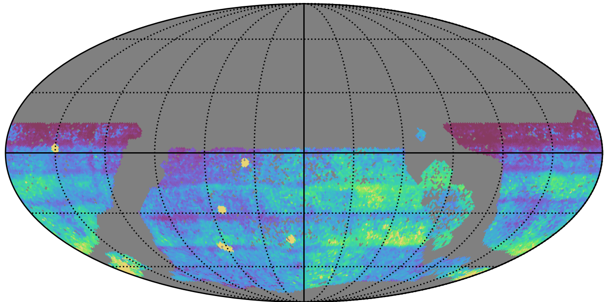
too_elab_heavy_r128_d3_griz_v3.4_10yrs WFD: 75th Percentile Intranight Timespan
