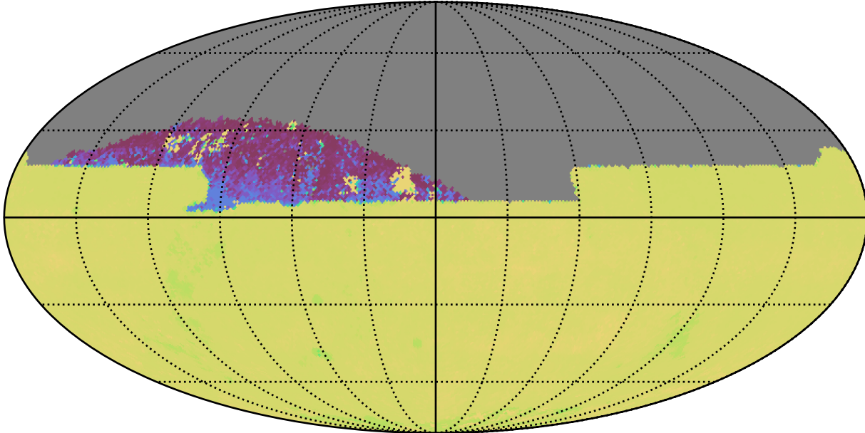
too_elab_heavy_r128_d3_griz_v3.4_10yrs All sky zy bands: 75th Percentile Intranight Timespan
