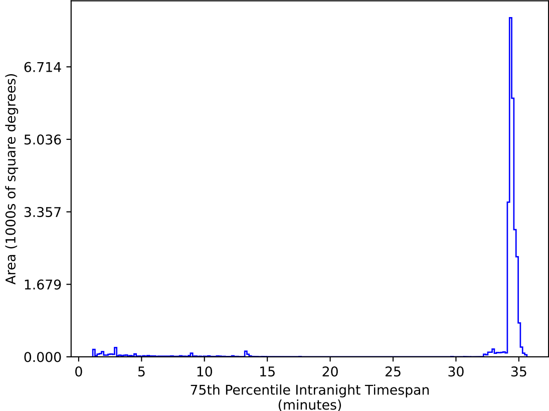
too_elab_heavy_r128_d3_griz_v3.4_10yrs All sky zy bands: 75th Percentile Intranight Timespan
