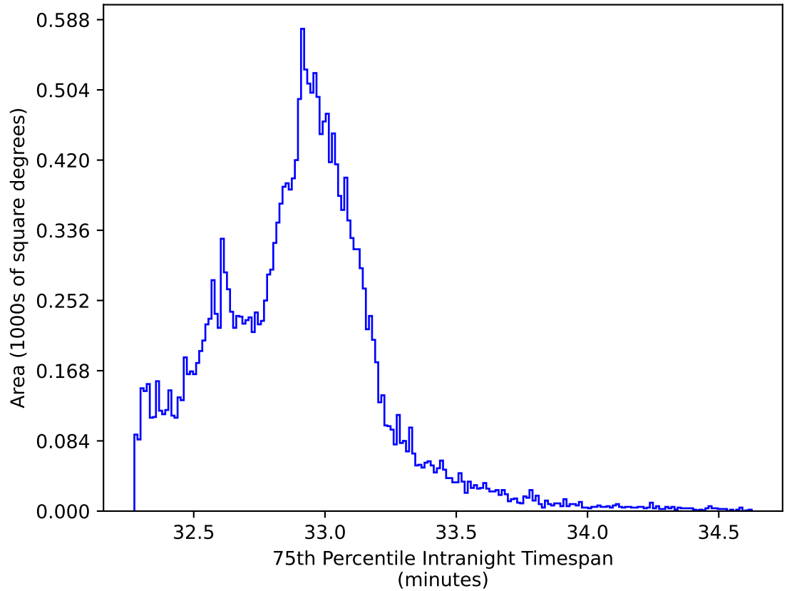
too_elab_heavy_r128_d3_griz_v3.4_10yrs All sky y band: 75th Percentile Intranight Timespan
