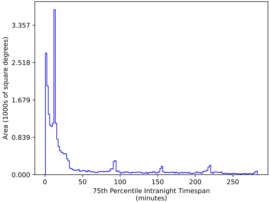
too_elab_heavy_r128_d3_griz_v3.4_10yrs All sky r band: 75th Percentile Intranight Timespan
