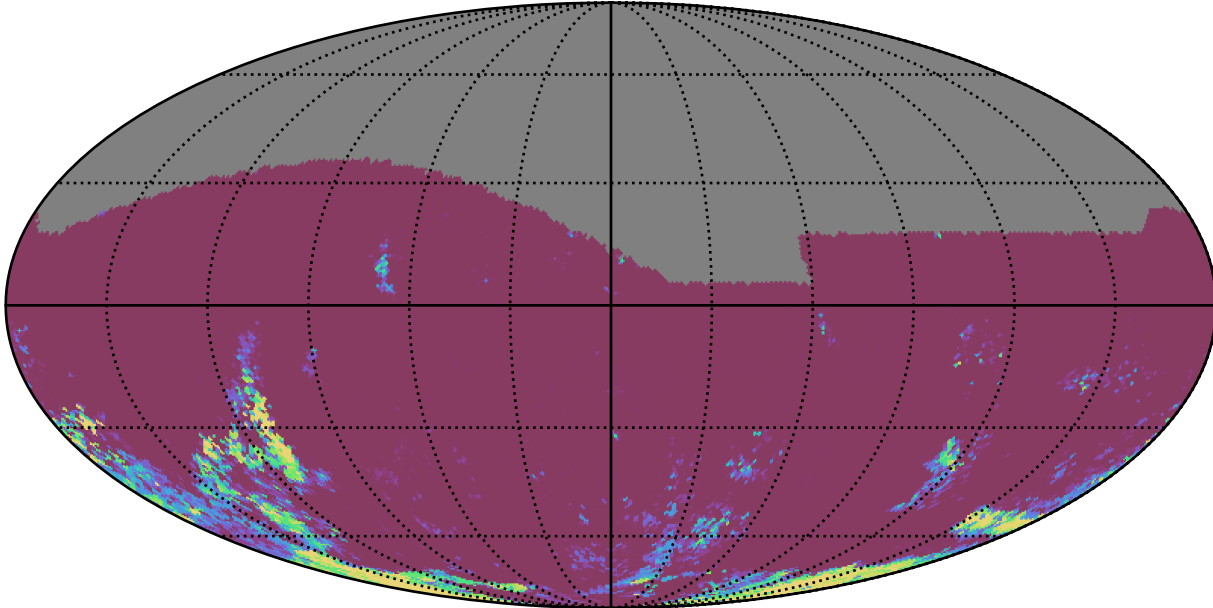
too_elab_heavy_r128_d3_griz_v3.4_10yrs All sky gr bands: 75th Percentile Intranight Timespan
