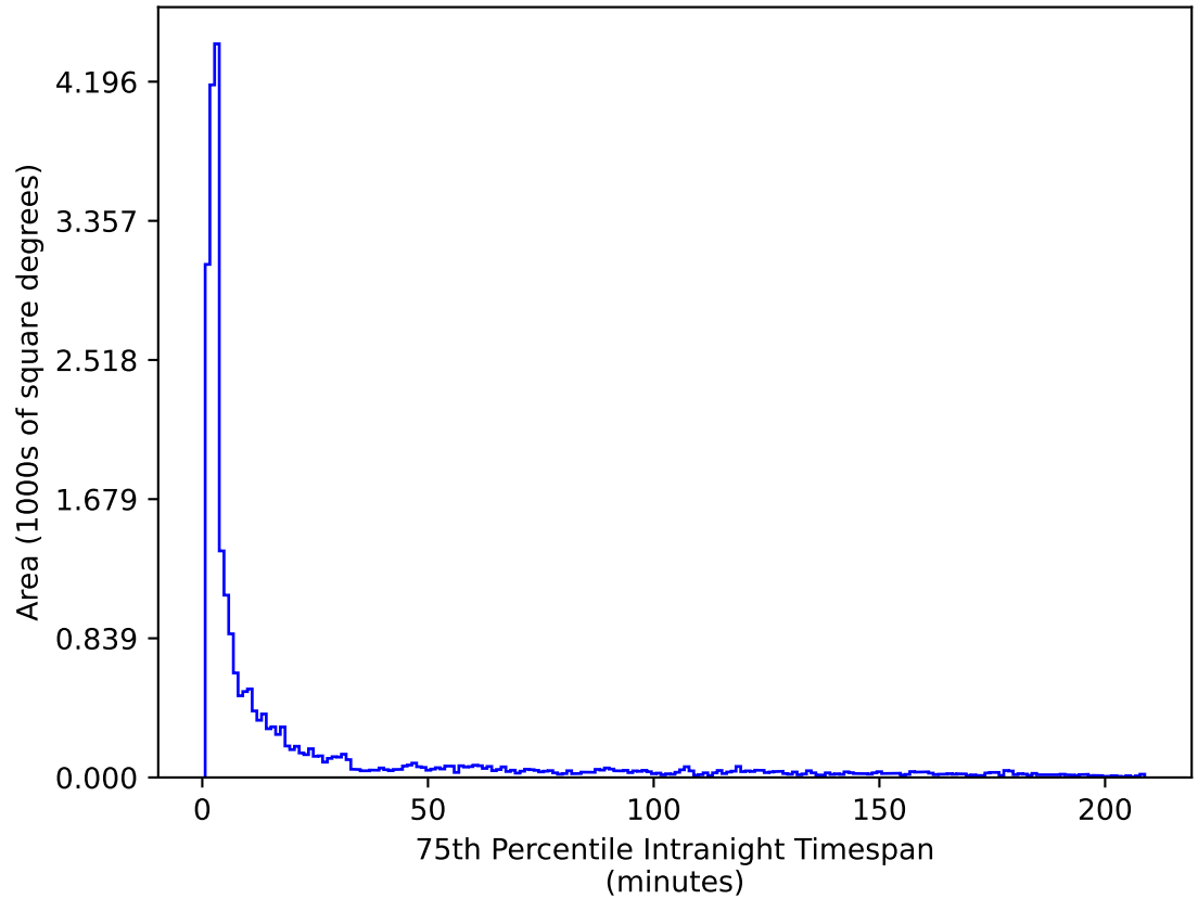
too_elab_heavy_r128_d3_griz_v3.4_10yrs All sky g band: 75th Percentile Intranight Timespan
