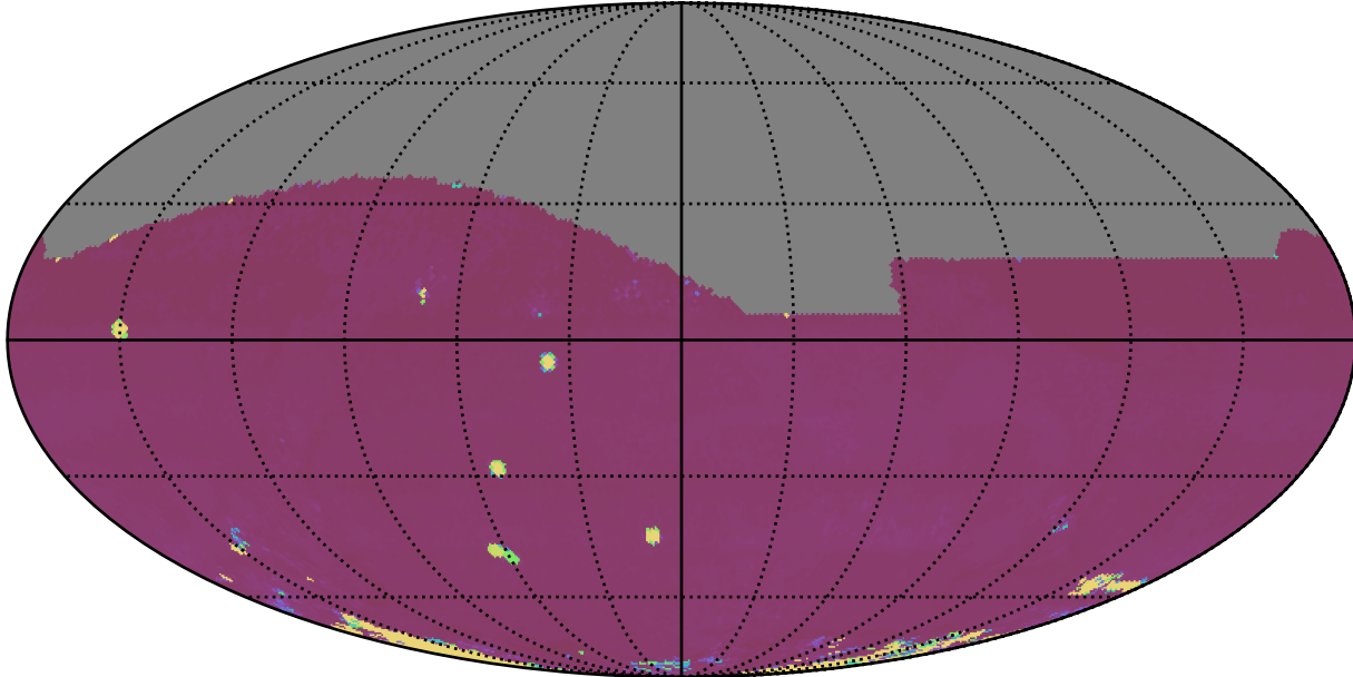
too_elab_heavy_r128_d3_griz_v3.4_10yrs All sky all bands: 75th Percentile Intranight Timespan
