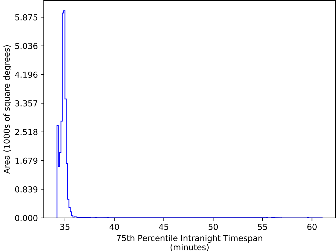
too_elab_heavy_r128_d3_griz_v3.4_10yrs All sky all bands: 75th Percentile Intranight Timespan
