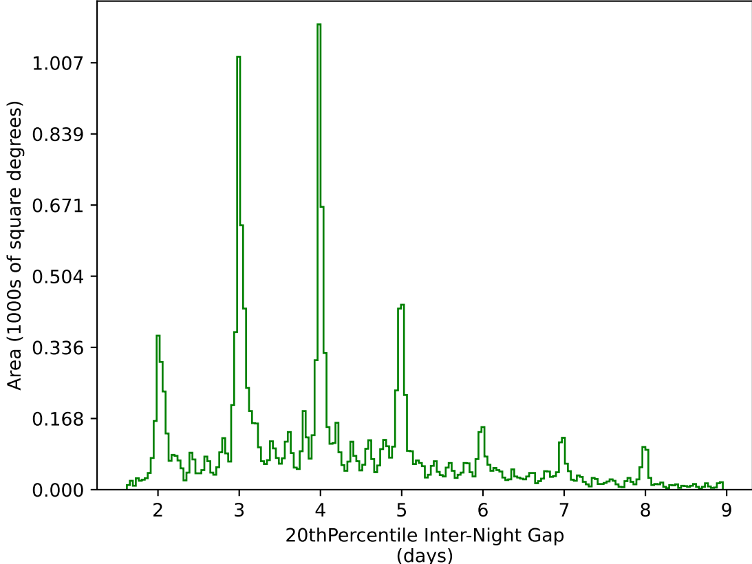
too_elab_heavy_r128_d3_griz_v3.4_10yrs WFD g band: 20thPercentile Inter-Night Gap
