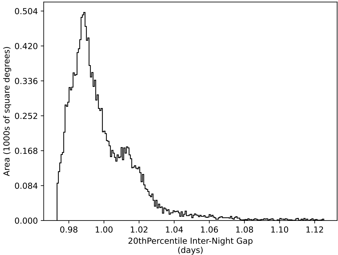
too_elab_heavy_r128_d3_griz_v3.4_10yrs WFD all bands: 20thPercentile Inter-Night Gap
