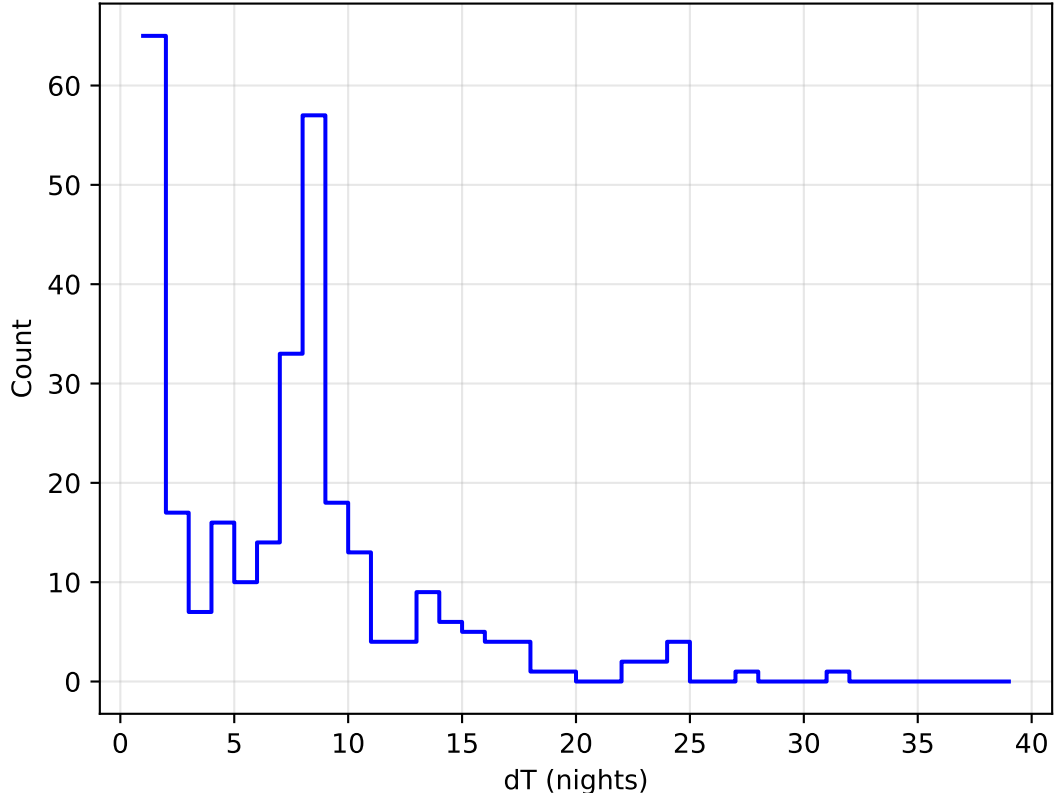
too_elab_heavy_r128_d3_griz_v3.4_10yrs all bands: DD:XMM_LSS Delta Nights Histogram
