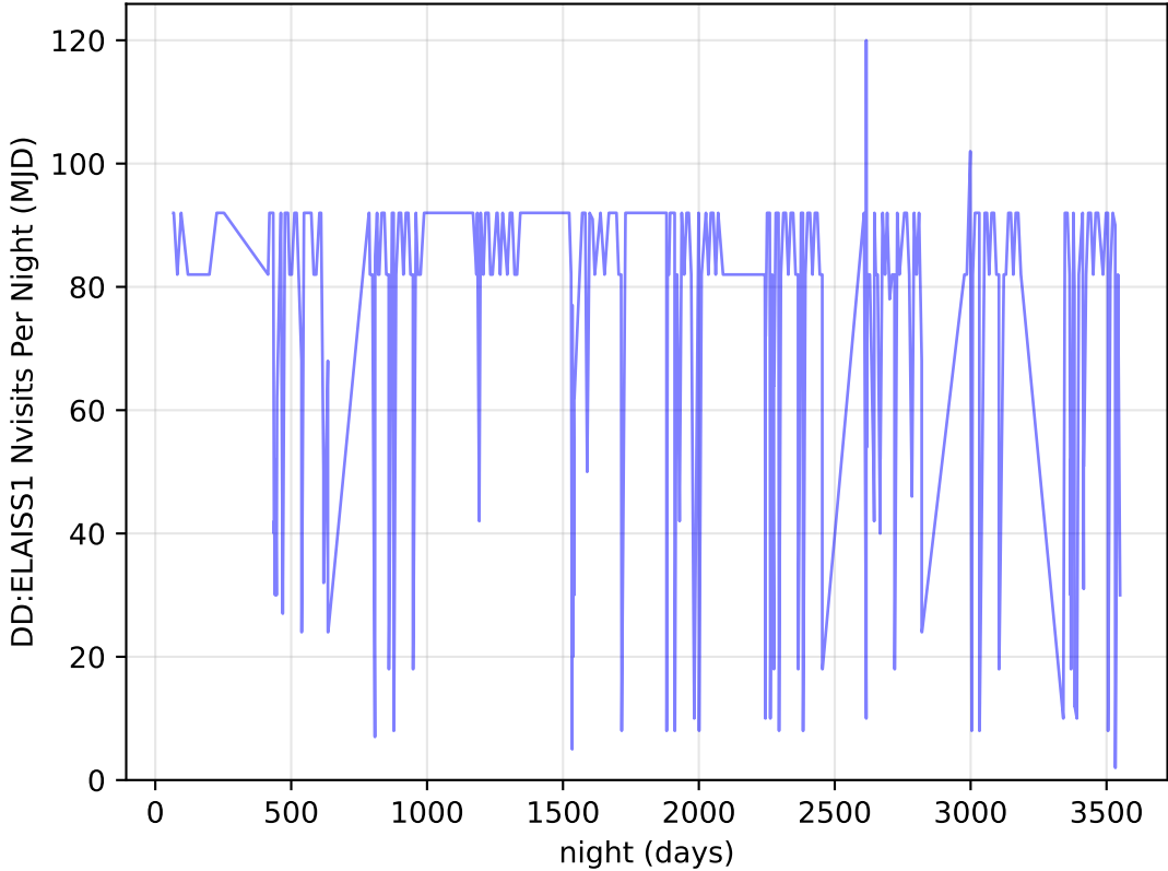
too_elab_heavy_r128_d3_griz_v3.4_10yrs all bands: DD:ELAISS1 Nvisits Per Night
