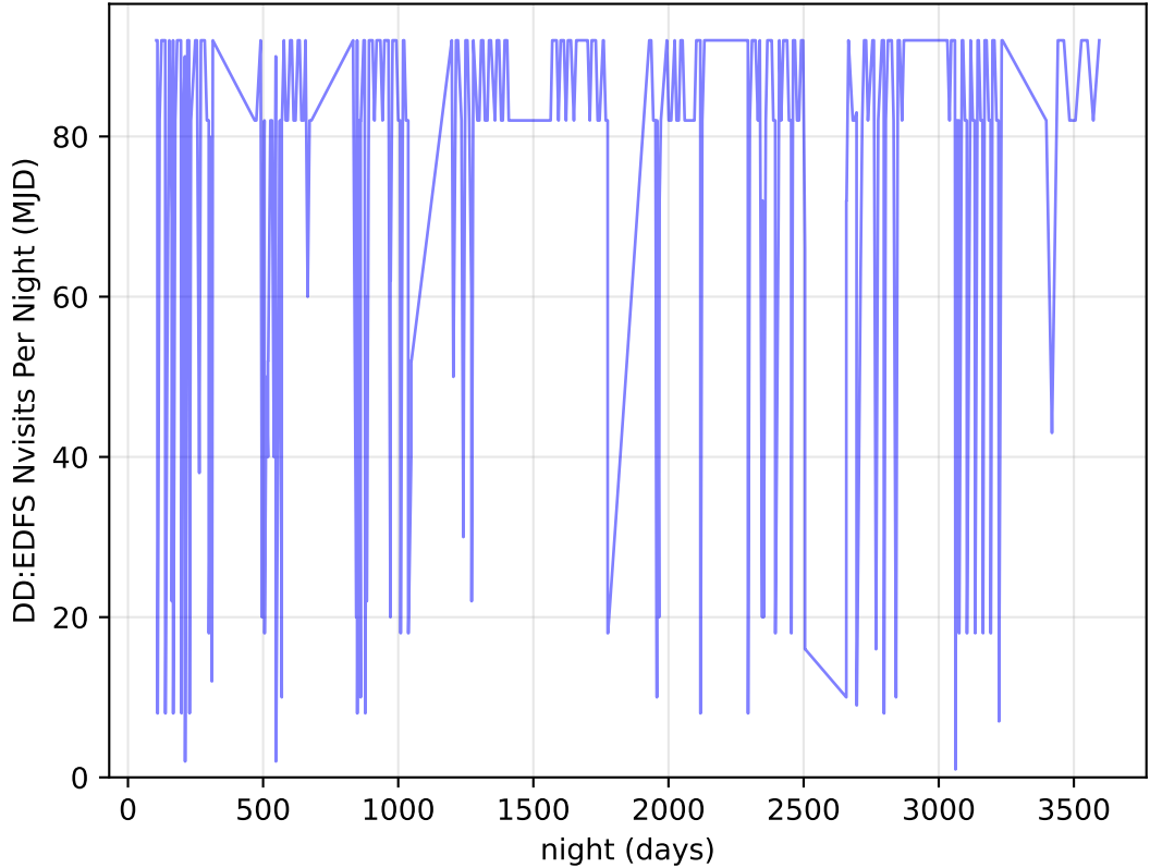
too_elab_heavy_r128_d3_griz_v3.4_10yrs all bands: DD:EDFS Nvisits Per Night
