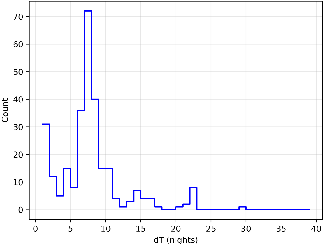
too_elab_heavy_r128_d3_griz_v3.4_10yrs all bands: DD:EDFS Delta Nights Histogram
