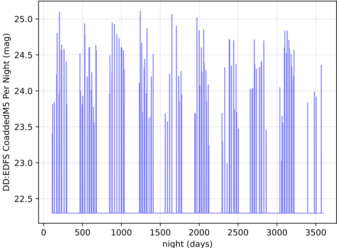
too_elab_heavy_r128_d3_griz_v3.4_10yrs u band: DD:EDFS CoaddedM5 Per Night
