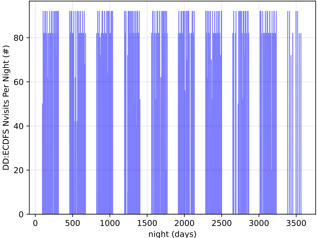
too_elab_heavy_r128_d3_griz_v3.4_10yrs all bands: DD:ECDFS Nvisits Per Night
